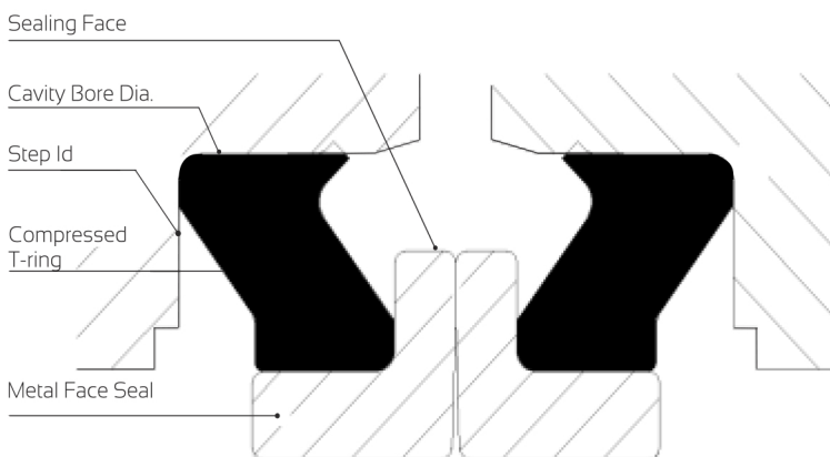
Assembled Condition
